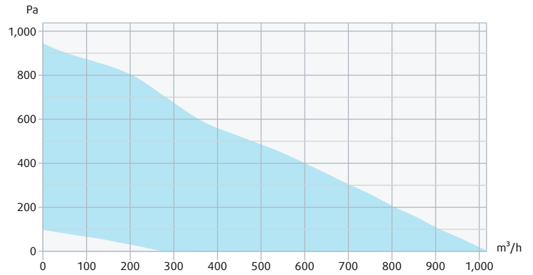
Extract - Performance curve
